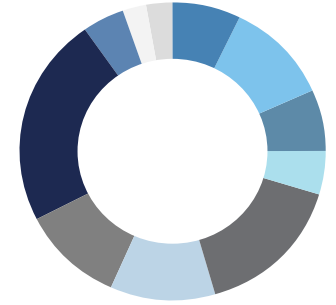
Benchmark
